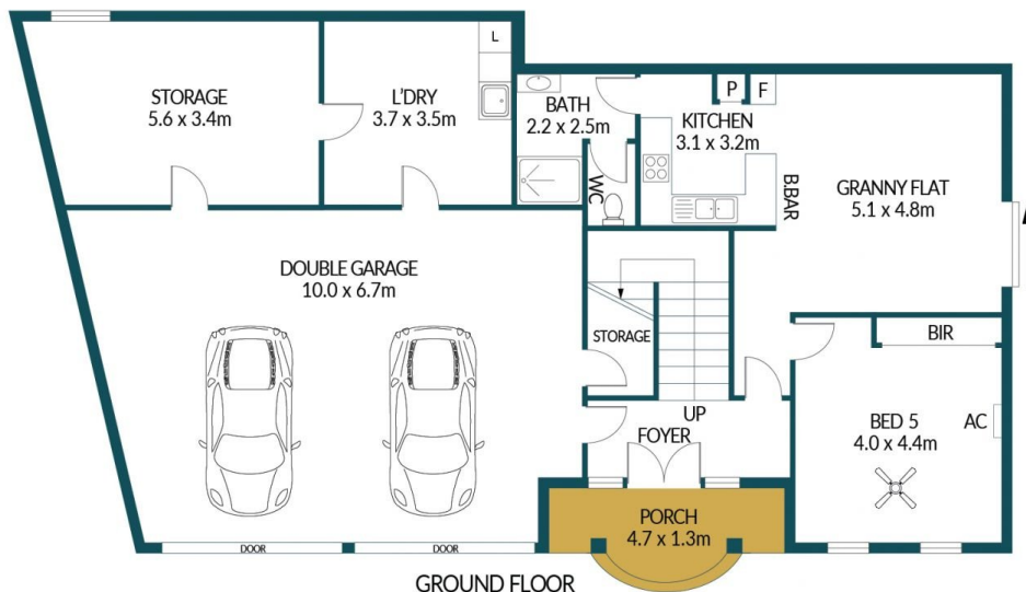
GROUND FLOOR
